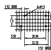
1 Form A (3.5 mm Pinning)
